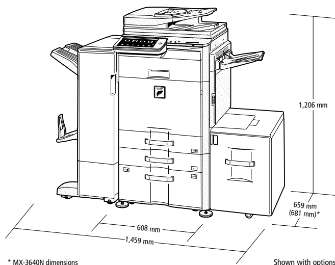
* MX-3640N dimensions
